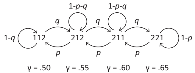
FIGURE 1: A Markov model representing transitions in a transitive (TAX) model between true preference states produced by changing the parameter \gamma . The dataset, Trans 1, was generated with p = q = 0.1
